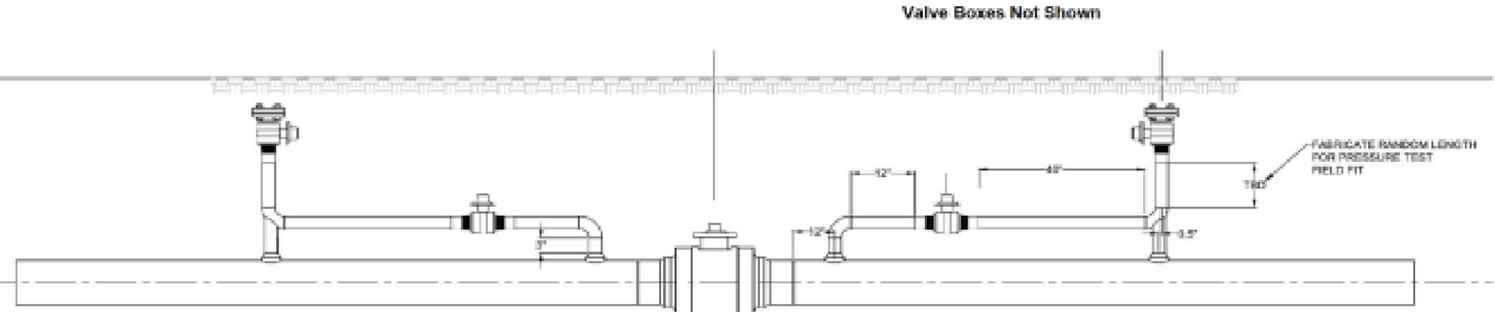
BLOCK AND VENT VALVES REV 3 - (1/8/2025)
