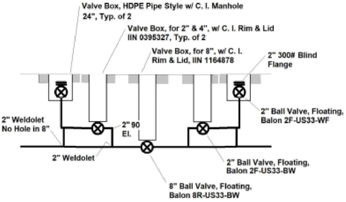
DETAIL "F" SHEET 6 OF 12 REV 3 - (1/8/2025)
